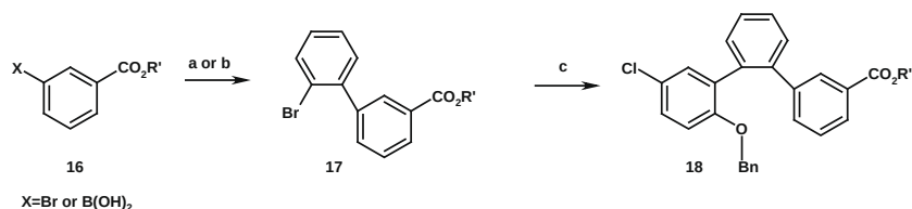
Scheme 3. Reagents and conditions: (a) 1,2-dibromobenzene, Pd(PPh 3 ) 4 , K 2 CO 3 , PhMe-EtOH, 90 °C. (b) (2-bromophenyl)boronic acid, Pd(PPh 3 ) 4 , K 2 CO 3 , PhMe-EtOH, 90 °C. (c) 15 , Pd(PPh 3 ) 4 , K 2 CO 3 , PhMe-EtOH, 90 °C.
