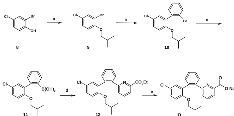
Scheme 1. Reagents and conditions: (a) iso-butyl bromide, K_2CO_3 , DMF, 80\text{ }^\circ\text{C} , 94%. (b) (2-bromophenyl)boronic acid, Pd(PPh_3)_4 , K_2CO_3 , PhMe-EtOH, 90\text{ }^\circ\text{C} , 47%. (c) n-BuLi , THF, -100\text{ }^\circ\text{C} ; B(Oi-Pr)_3 , -78\text{ }^\circ\text{C} –rt.; 2 M HCl, 83%. (d) Ethyl 6-bromo-2-pyridinecarboxylate, Pd(PPh_3)_4 , K_2CO_3 , PhMe-EtOH, 90\text{ }^\circ\text{C} , 100%. (e) EtOH, 2 M NaOH, 96%.
