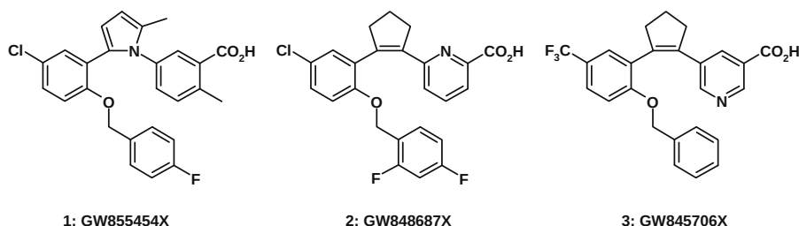
Figure 1. Selected published GSK EP 1 receptor antagonists GW855454X ( 1 ), GW848687X ( 2 ) and GW845706X ( 3 ).
