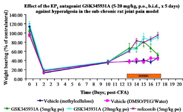
Figure 3. Effect of 5 mg/kg p.o. b.i.d. and 20 mg/kg p.o. b.i.d. GSK345931A ( 7i ) in the sub-chronic rat joint pain assay versus vehicle (methylcellulose) and positive control (rofecoxib 5 mg/kg p.o.) and positive control vehicle (DMSO/PEG/water).
